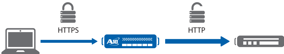
Figure 7: End-to-end SSL Overview
